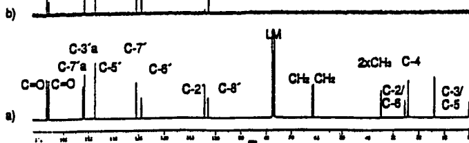
Figure 1. 13 C-nmr spectra (62.89 MHz, Bruker WM 250) in trichlorodeuteriomethane for compound 4 : a) 1 H-noise decoupled spectrum; b) 13 C{ 1 H}-NOE difference spectrum obtained by selective irradiation of H-N(4') respectively
